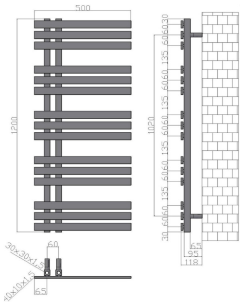
1200x500mm
