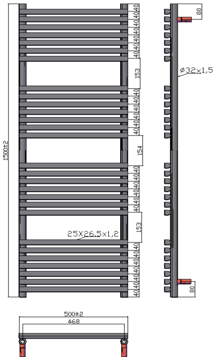
1500X500M
