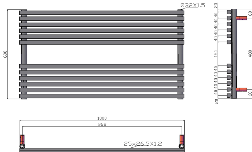
600X1000MM
